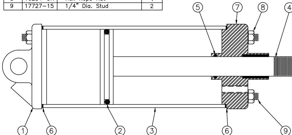
BUCK TRANSFER CYLINDER (Part No. A-5130)
