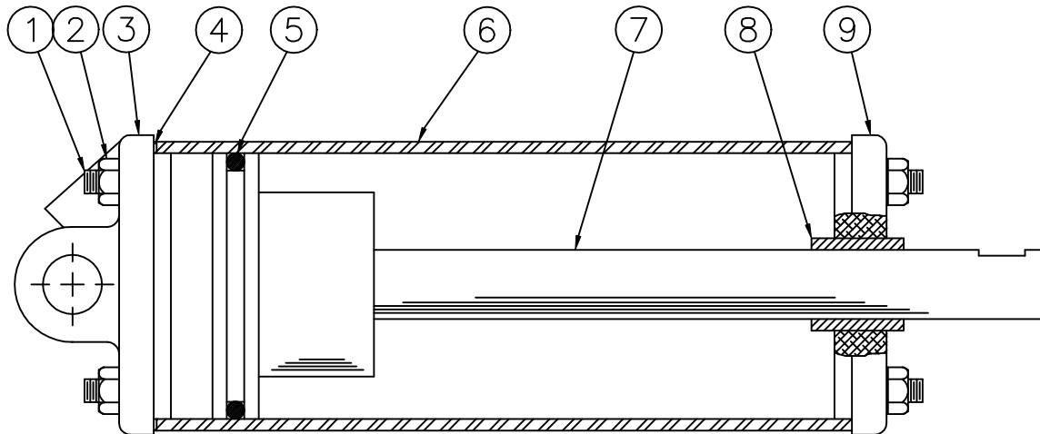
HEAD CLOSING CYLINDER (Part No. A-5315)
